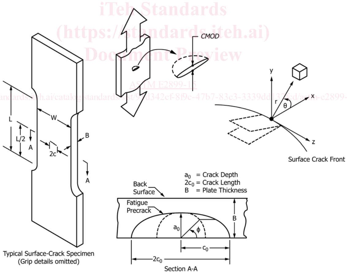
FIG. 1 Test Specimen and Crack Configurations
