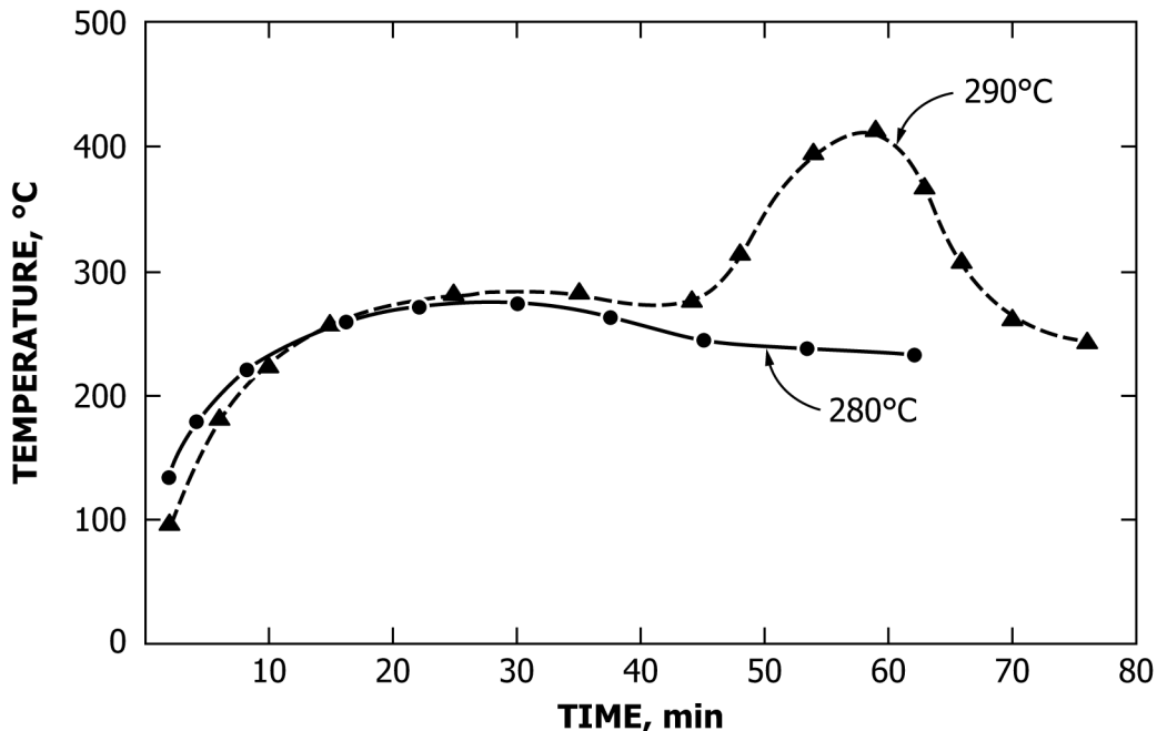
FIG. 4 Test Data Showing Nonignition at Set Temperature of 280^\circ\text{C} and Ignition at Set Temperature of 290^\circ\text{C}
