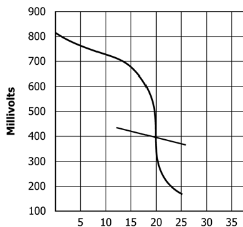
NOTE 1—Twenty millilitres of 2.51 g/L KCN titrated with \text{AgNO}_3 . FIG. 1 Typical Titration Curve Standardizing KCN Solution
