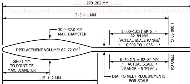
FIG. 2 Soil Hydrometers
