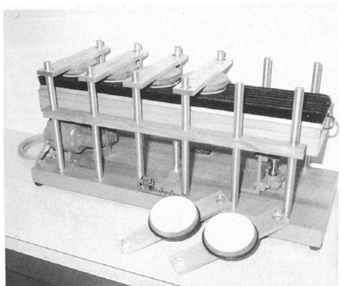
FIG. 1 Brush Pilling Tester
