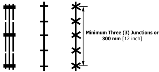
FIG. 12 Specimen Dimensions for Method A
