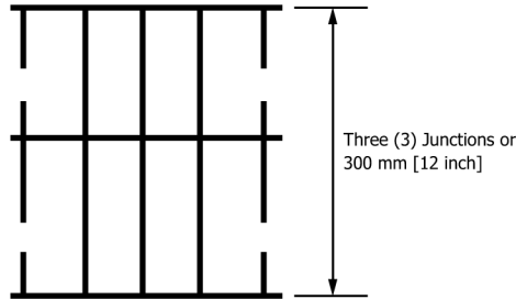
FIG. 23 Specimen Dimensions for Methods B and C
