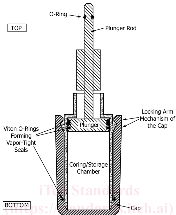
FIG. 3 Components of the En-Miniature Core Sampler
