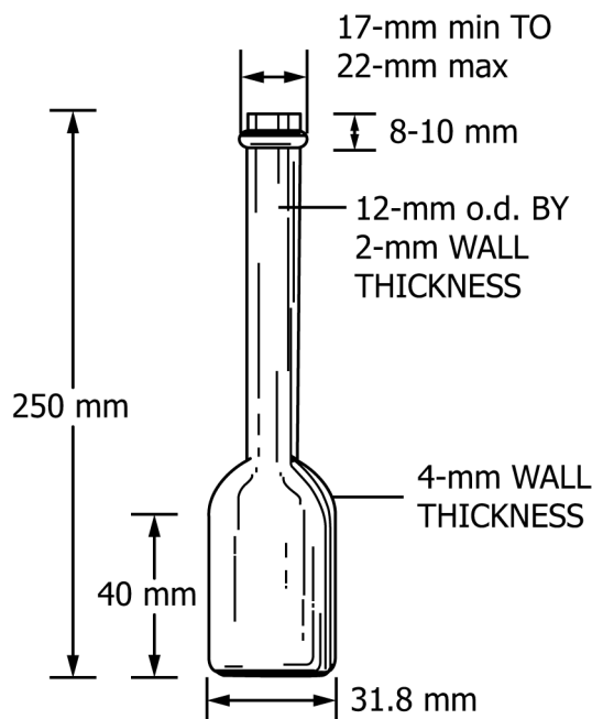
FIG. 1 Sealed-Reflex Dissolution Tube
