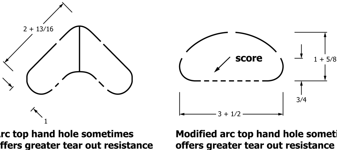
FIG. 1 Common Hand Hole Types
