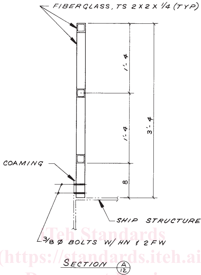
FIG. 2 Steel Coaming
