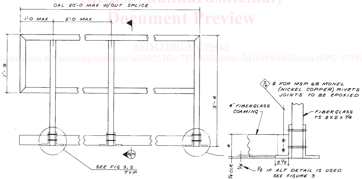
FIG. 1 Fiberglass Coaming
