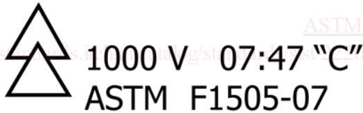
FIG. 7 Example of Markings on Insulating Materials, Consisting of (see 5.6.2): The double triangle symbol, the voltage rating for the tool, an example of a manufacturer's date code (YR:WK), the low temperature (−40°C) symbol, and the relevant ASTM standard
