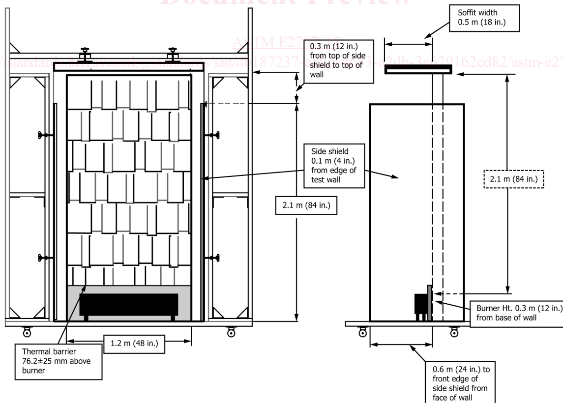
FIG. 1 Test Fixture
