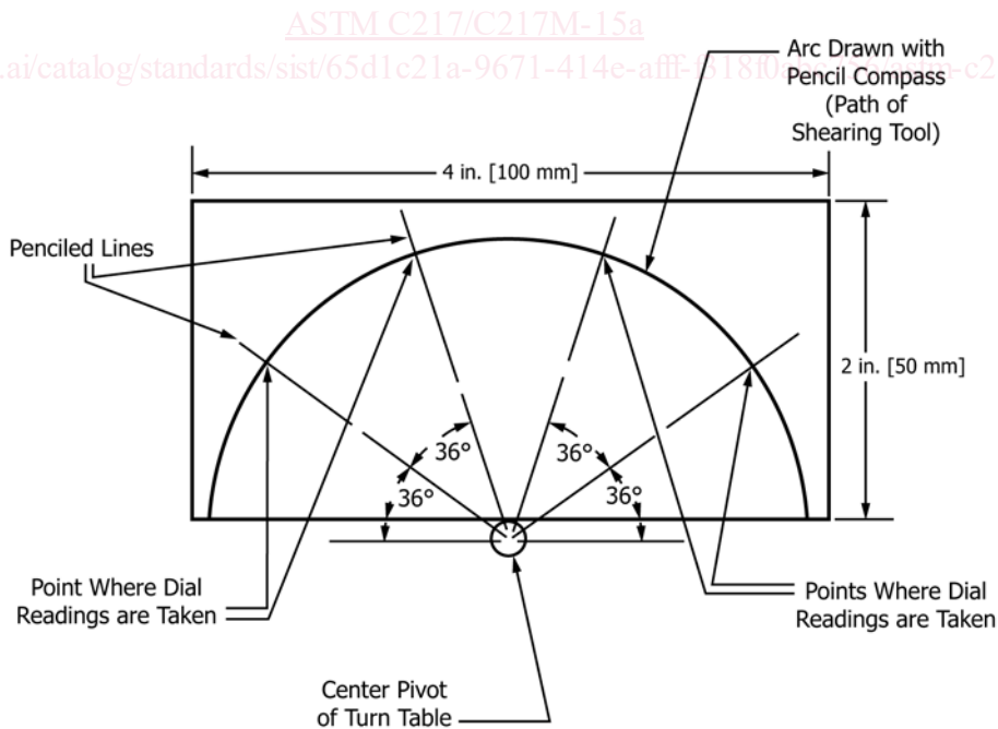
FIG. 2 Diagram of Slate Specimen Prepared for Test with Shear/Scratch Tester
