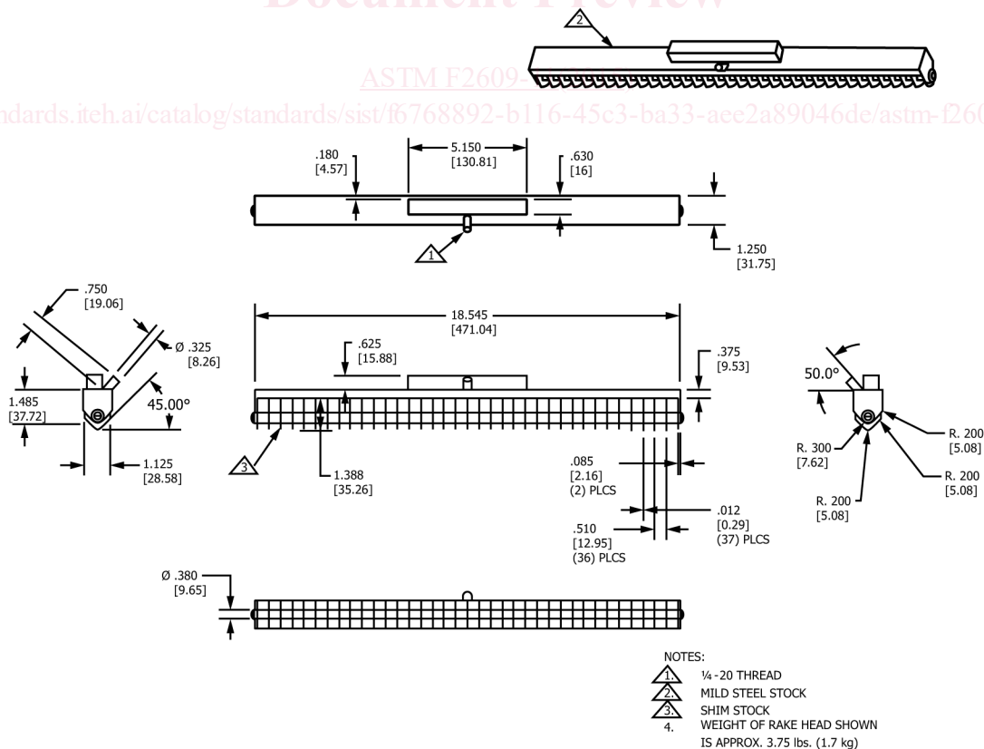
FIG. 1 Rake Head
