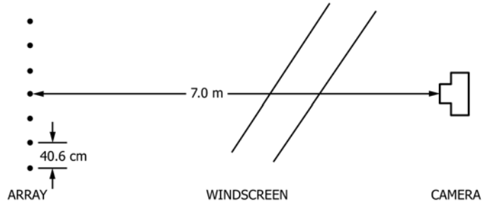
FIG. 2 Schematic Drawing of Component Layout for Measuring Multiple Imaging Angular Displacement
