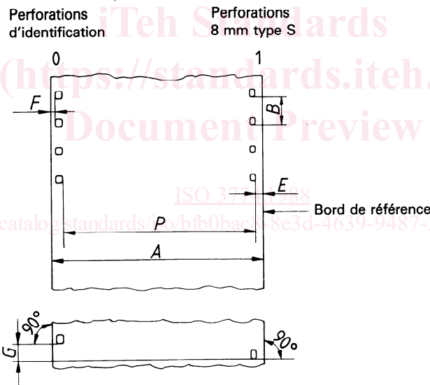
Figure 2 — Film perforé 1-0
