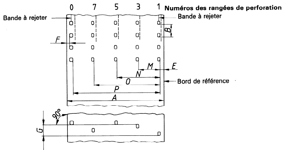
Figure 1 — Film perforé 1-3-5-7-0
