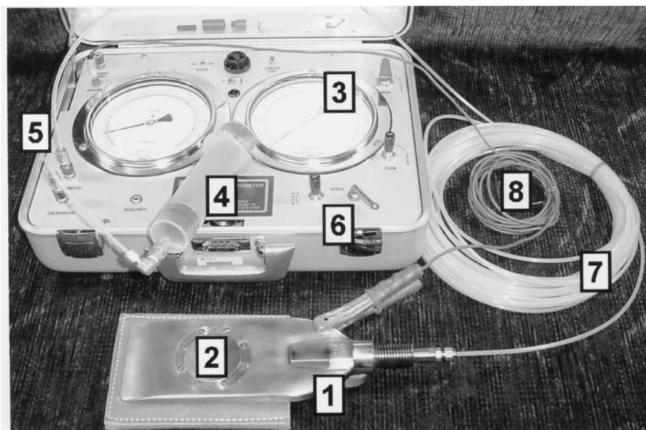
FIG. 1 DMT Equipment
