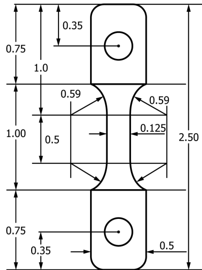
FIG. 2 Specimen Geometry—Test Specimen Dimensions
