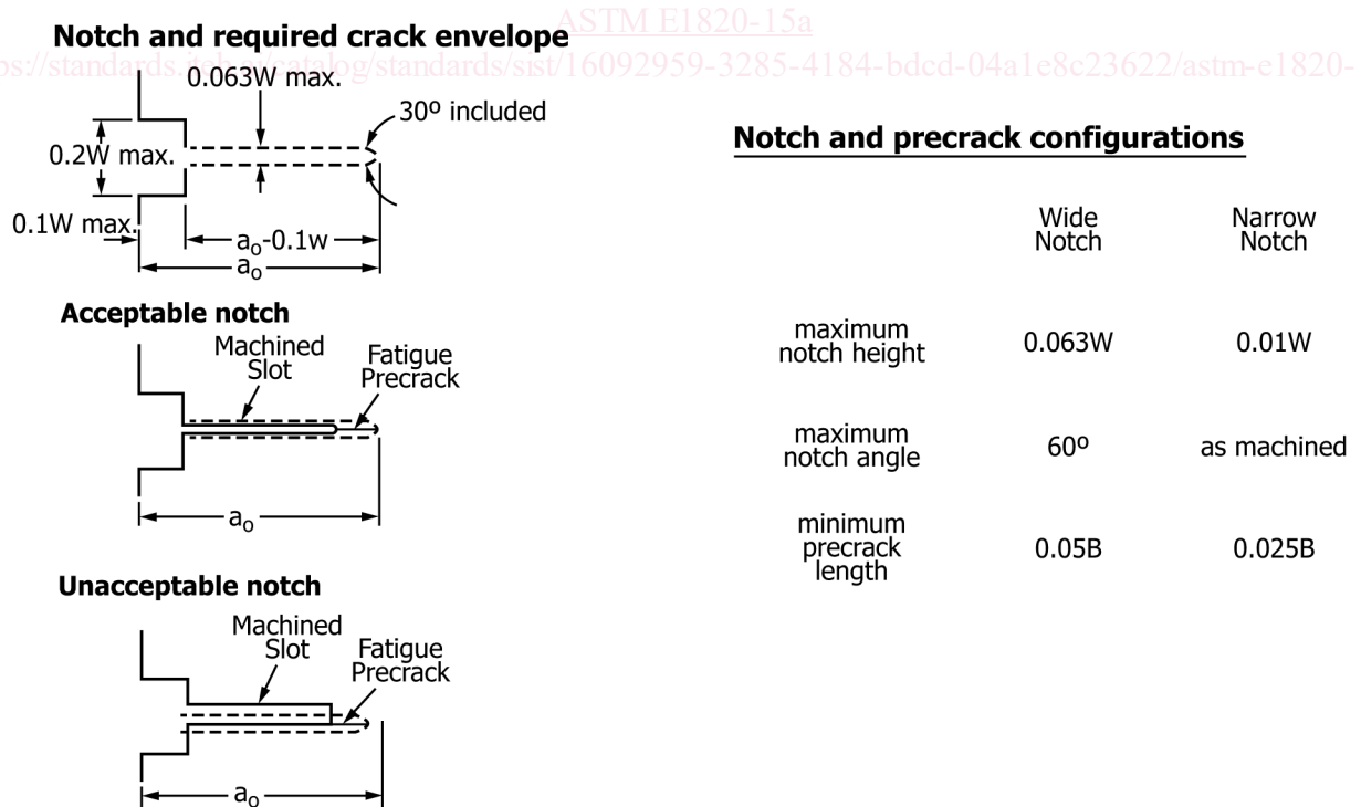
FIG. 7 Envelope of Fatigue Crack and Crack Starter Notches
