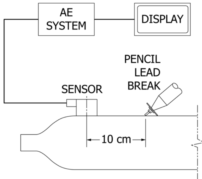
FIG. 1 Illustration of Peak Amplitude Performance Verification
