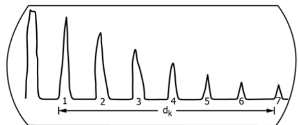
FIG. 1 Initial Pulse and 7 Back Echoes
