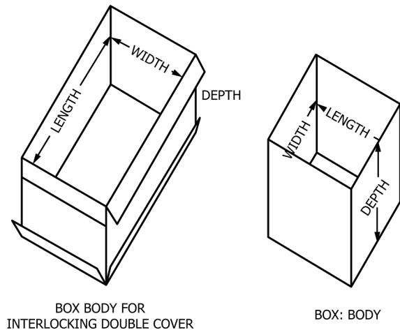
FIG. 1 Fiberboard Box Dimensioning
