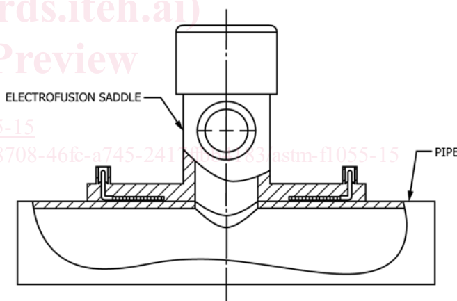
FIG. 3 Correct Wire Termination—Saddle Fitting
