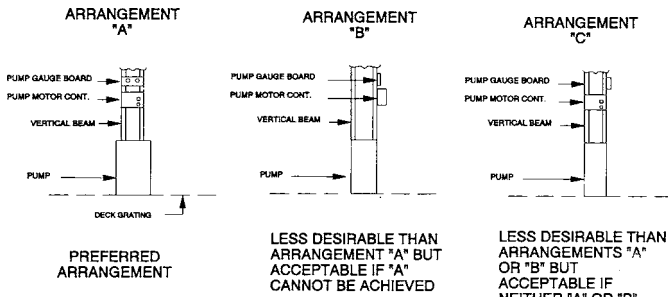
FIG. 4 Example of Control/Display/Equipment Relationship in Machinery Space with Pump, Motor Controller, and Gage Board Located at Vertical Beam
