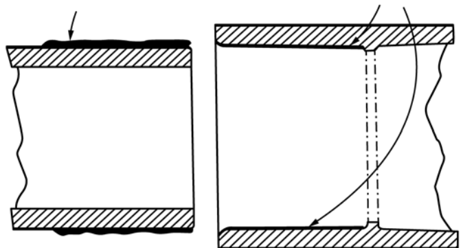
FIG. 2 Solvent Cement Coatings of Appropriate Thickness
