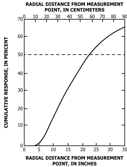
FIG. 2 Cumulative Response Versus Radial Distance for a Typical Electromagnetic-Induction Probe Showing Depth of Investigation Exploration and Radial Focusing (2)
