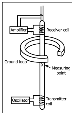
FIG. 1 Electromagnetic-Induction Logging System (1)
