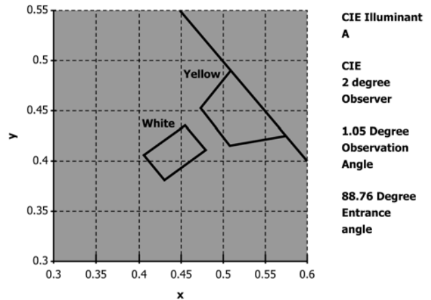
FIG. 2 Nighttime Chromaticity of Pavement Markings
