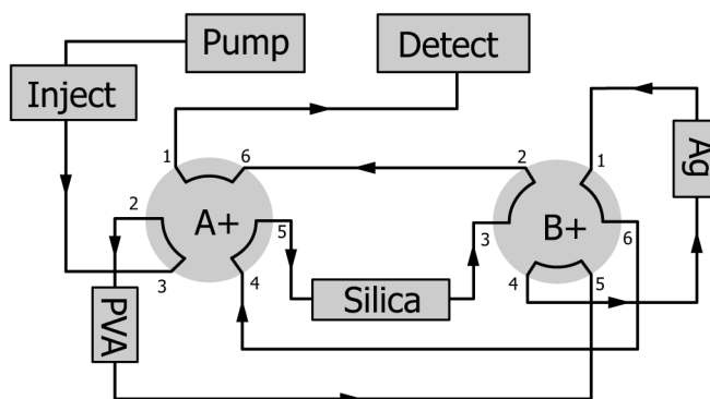
FIG. 4 Valve Position EA—High Resolution of Aromatics, Step 5
