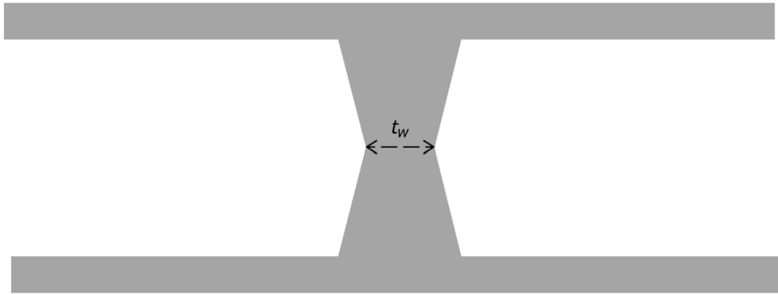
NOTE 1—If t_w is less than 0.75 in. [19 mm] over the entire height of the web, disregard entire area of that web when determining minimum web area. FIG. A1.1 Example of Web with Irregular Cross-section—Plan View
