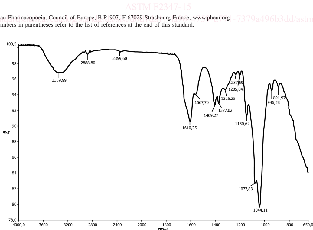
FIG. 1 FT-IR Spectrum of Hyaluronan, Sodium Salt Using Horizontal Attenuated Total Reflectance (HATR)
