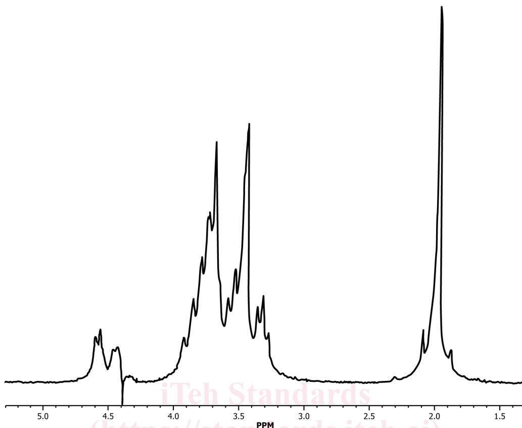
FIG. 2 ^1\text{H} NMR Spectrum of Hyaluronan from Rooster Comb (Mw ~700 000)
