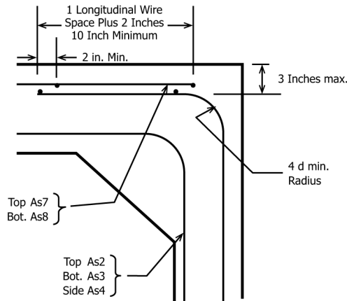
FIG. 6 Detail Option
