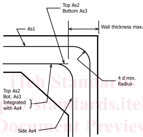
FIG. 7 Alternate Detail
