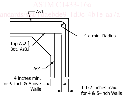
FIG. 3 Detail Inner Reinforcement
