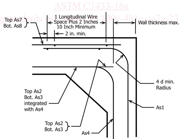
FIG. 8 Alternate Detail
