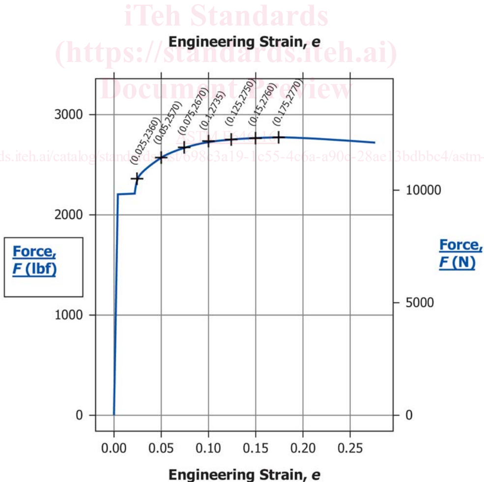
FIG. 2 Example Showing Load-Strain Data Pairs: material with initial discontinuous yielding region. These data pairs are used for a sample calculation in Appendix X1
