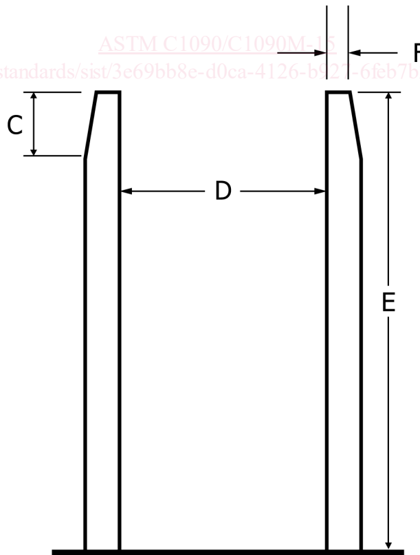
FIG. 1 Cylinder Mold with Machined (Tapered) Top Edge (see Table 1 for dimensions)
