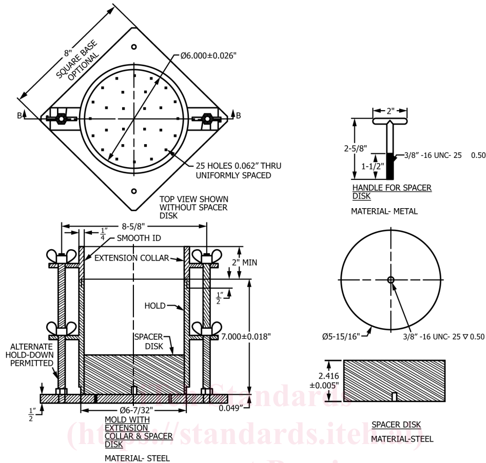
FIG. 1 Bearing Ratio Test Apparatus Mold with Extension Collar and Spacer Disk
