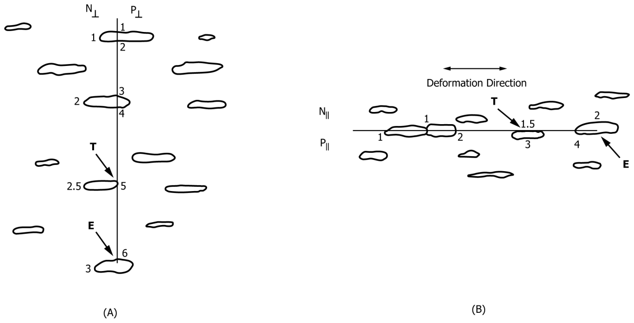
NOTE 1—The test grid lines have been shown oriented perpendicular (A) to the deformation axis and parallel (B) to the deformation axis. The counts for N_{\perp} , N_{\parallel} , P_{\perp} , and P_{\parallel} are shown for counts made from top to bottom (A) or from left to right (B). NOTE 2— T indicates a tangent hit and E indicates that the grid line ended within the particle; both situations are handled as shown.
