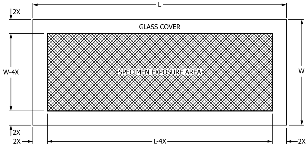
FIG. 2 Sample Exposure Area Diagram
