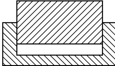
FIG. 3 Positive-Type Mold
