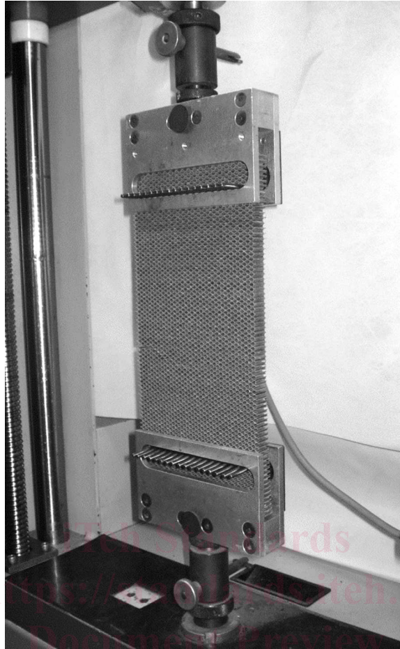
FIG. 1 Honeycomb Core Tensile-Node Bond Strength Test Setup
