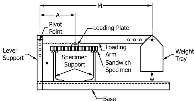
FIG. 1 Creep Test Apparatus and Loading System
