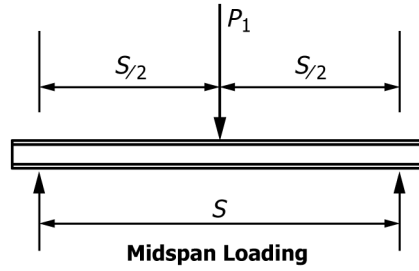
(a) 3-Point Loading (Standard Configuration)
