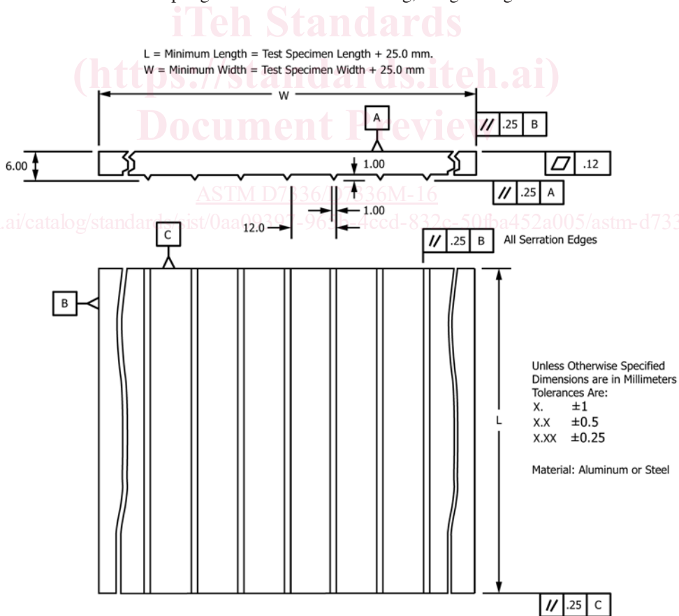
FIG. 3 Representative Serrated Plate for Honeycomb Core Material Pre-Crushing (SI Version)
