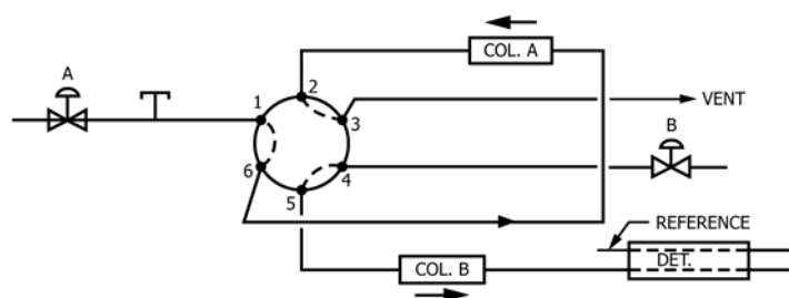
FIG. 2 Valve Backflush
