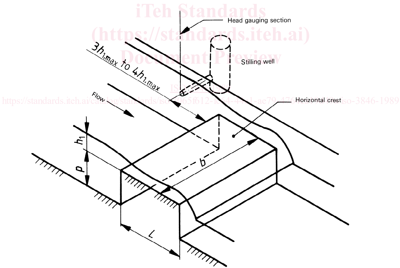
Figure 1 — Rectangular broad-crested weir
