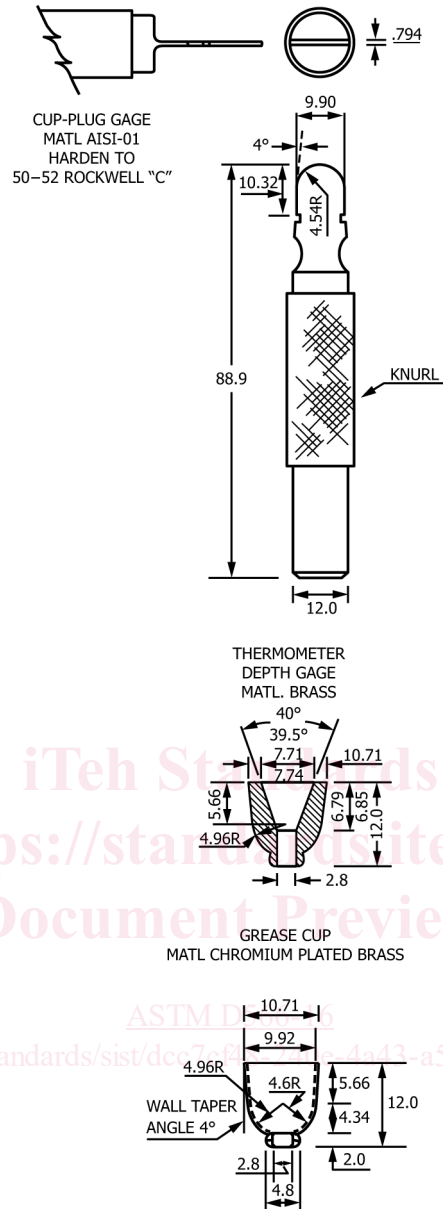
FIG. 1 Plug Gage, Gauge, Depth Gage, Gauge, and Grease Cup
