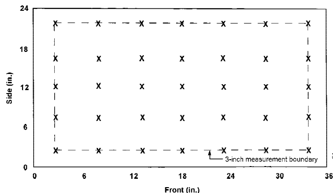
FIG. 2 Sample Placement of Thermocouples on a 3 by 2-ft (0.6 by 0.9-m) Griddle
