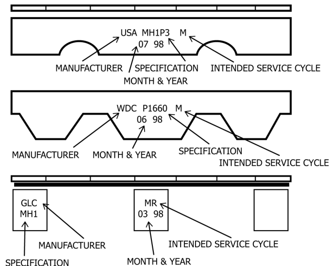
FIG. 23 Marking Requirements (Location of Markings Optional)
