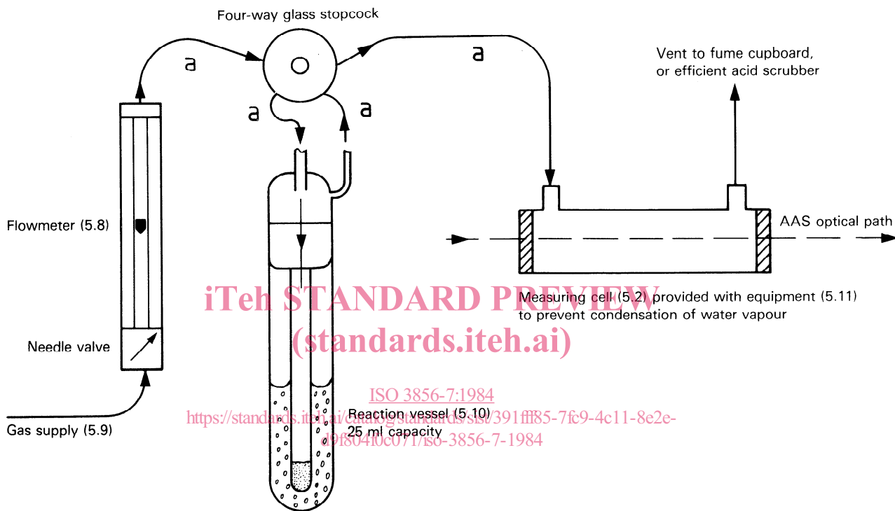
Figure 2 — Example of apparatus for the determination of mercury by flameless atomic absorption spectrometry
