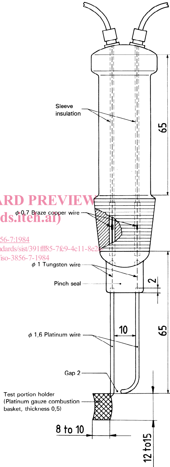
Figure 1 — Firing adapter
