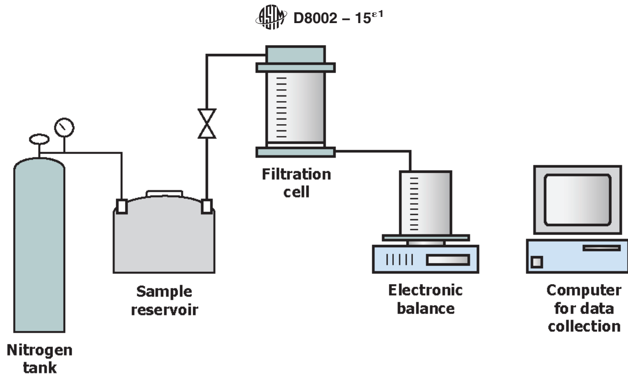
FIG. 2 Representative Apparatus for Measuring MFI at Constant Pressure with a Pressure Vessel
