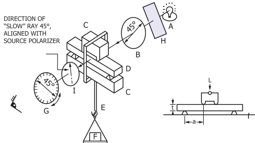
FIG. 5 Schematic of 4-Point Beam Loading System
