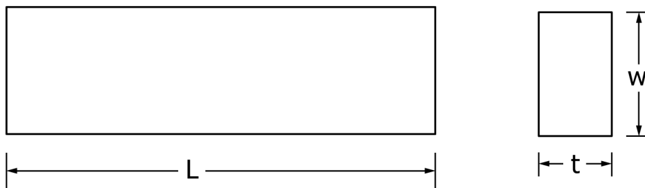
(a) Beam-Stressing-and-Polarimeter-Arrangement FIG. 7 Rectangular Compression Specimen
