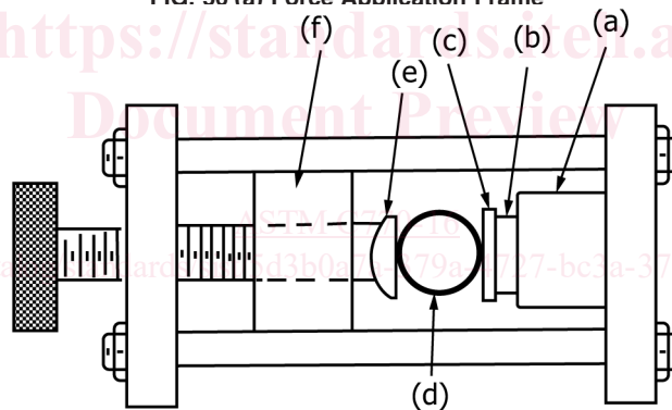
FIG. 56 (a) Force Application Frame
