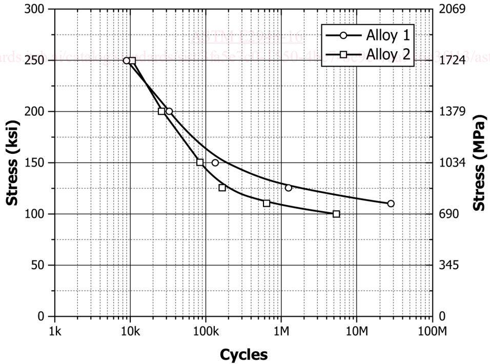
FIG. 5 Typical Stress-Life Diagram for Alloy 1 and Alloy 2.
