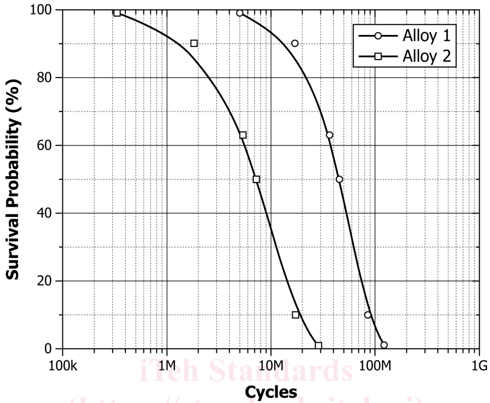
FIG. 4 Typical Survival Probability Graph of Fatigue Data for Alloy 1 and Alloy 2
